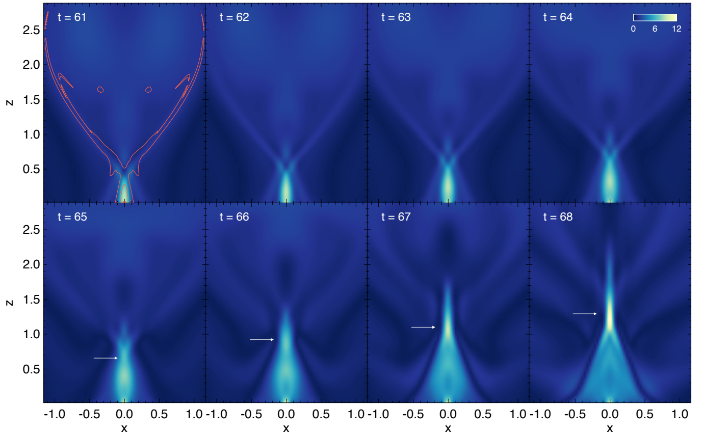
Figure 9. Current structures in the reconnection region during 61 \leq t \leq 68 . Each sub-panel shows the distribution of dimensionless J/B on the plane y = 0 . The colorbar for J/B in all sub-panels is displayed at the upper right corner. The red contours in first sub-panel show the outlines of QSLs at t = 61 . The white arrows mark the forming current sheet in the reconnection region.
