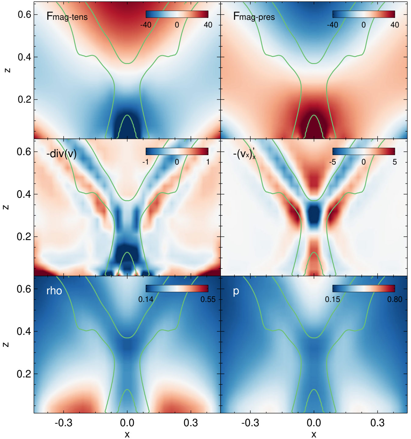
Figure 7. Some parameters related to force analysis on the plane y = 0 at t = 58 . They are in order as follows: z -component of magnetic tension force ( F_{mag-tens} ), z -component of magnetic pressure gradient force ( F_{mag-pres} ), negative divergence of velocity ( -\text{div}(v) ), negative partial derivative of x -component of velocity to x ( -(v_x)'_x ), mass density ( \rho ), and thermal pressure ( p ). All parameters are in dimensionless units. The positive -\text{div}(v) and -(v_x)'_x at the two flanks of the flux rope bottom clearly show the compression caused by the reconnection inflow. The green curves represent contours of the QSLs.
