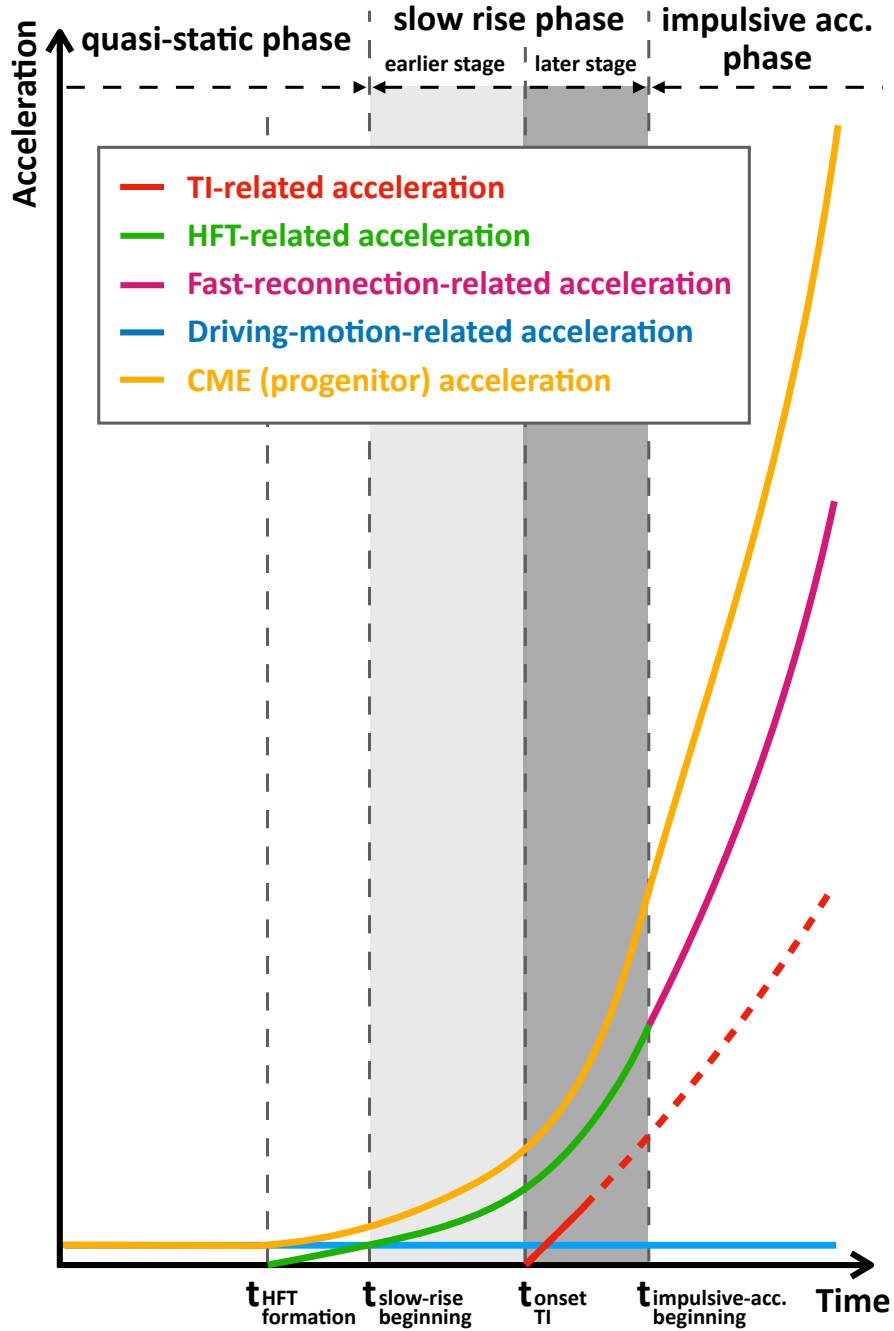
Figure 12. Physical processes as disclosed by the kinematics of the CME progenitor and CME. The yellow curve represents the acceleration of the CME (progenitor). The red, green, purple, blue curves show the four accelerations contributed by the torus instability, the HFT reconnection, the fast magnetic reconnection, and the driving motion, respectively. The onset times of the HFT, the slow rise, the torus instability, and the impulsive acceleration (abbreviated as acc.) of the CME are displayed by four dashed lines and labeled as t_{\text{HFT-formation}} , t_{\text{slow-rise-beginning}} , t_{\text{onset-TI}} , and t_{\text{impulsive-acc.-beginning}} , respectively. In our simulation, these four onset times correspond to t = 46 , t = 52 , a moment during the period 59 \leq t < 63 , and t = 65 , respectively. The light grey and dark grey regions show the earlier stage and the later stage of the slow rise phase/CME initiation process, respectively. The red curve is dashed during a part of the slow rise phase and the impulsive acceleration phase, indicating that the dominant mechanism for the acceleration is unknown whether it is torus instability or magnetic reconnection in these periods.
