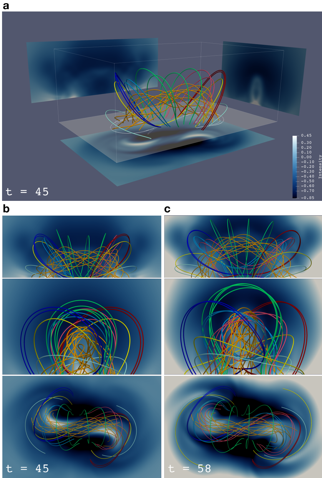
Figure 10. Magnetic field lines and synthetic EUV images at the AIA 335 Å. (a) Same as Fig. 2a but for t = 45 . (b) Three side views of field lines and percentage difference images at t = 45 . (c) Same as the panel b but for t = 58 .
