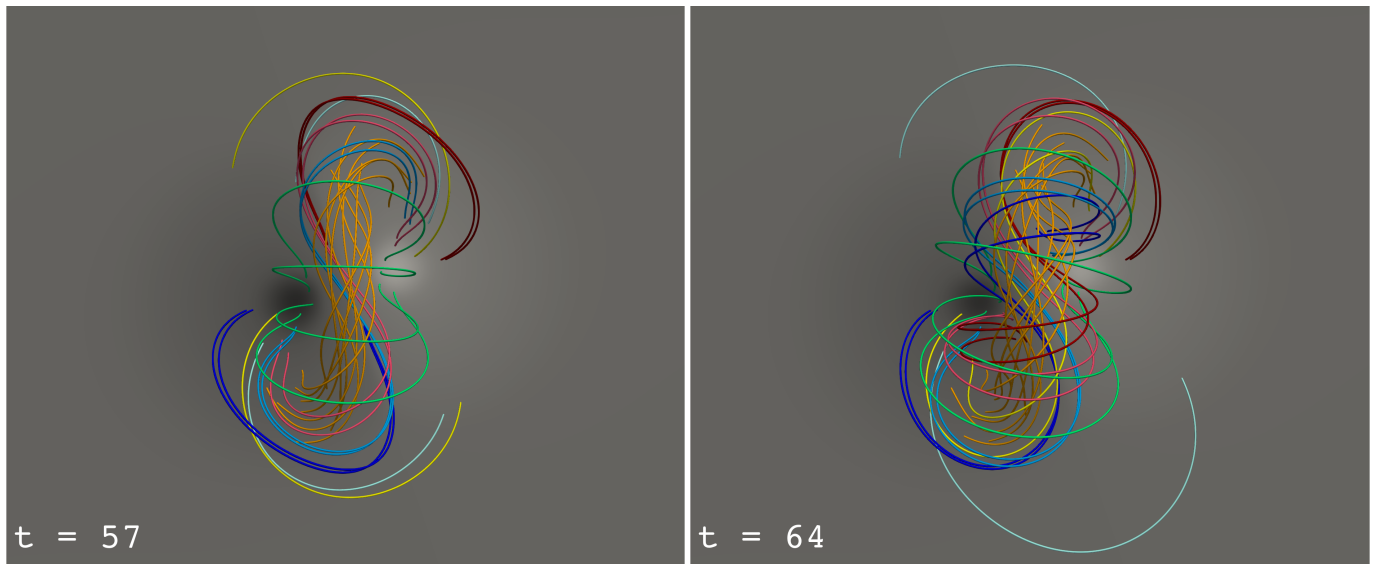
Figure S2. Top views of magnetic field lines in Fig. 2b. The left panel is at t = 57 and the right panel is at t = 64 . The vertical direction is the y-direction.
