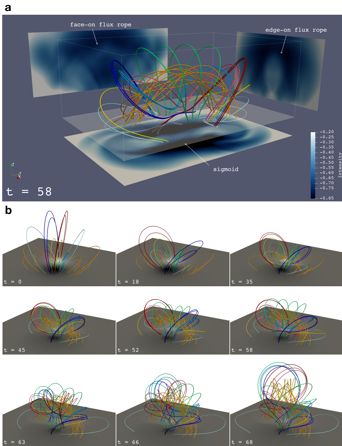
Figure 2. Overview of the formation and eruption of the modelled flux rope. (a) Field lines and percentage difference of synthetic EUV images at the AIA 335 Å at t = 58 . The left, right, bottom images are the synthetic images observed from x , y , and z directions, respectively. The translucent surface corresponds to cell-center bottom surface and the box is used for integrating the emissivity. The white contours on the bottom surface represent those of QSL footprints. The three side views of this panel are shown in Fig. 10c. (b) Evolution of magnetic field lines. The sub-panel at t = 58 is the same as panel a. The cyan field line at t = 35 and the yellow field line at t = 45 are tangent to the bottom surface at their dips, representing the field lines traced from the BP. The light blue and light red field lines at t = 52 and the dark blue and dark red field lines at t = 58 exhibit those passing through the HFT. The cell-center bottom surface shows the distribution of B_z . White (black) represents the positive (negative) polarity. The scale of B_z is the same in each panel. An animation of panel b is available, showing the evolution of field lines from t = 0 to t = 68 in the simulation. The duration of the animation is 23 s.
