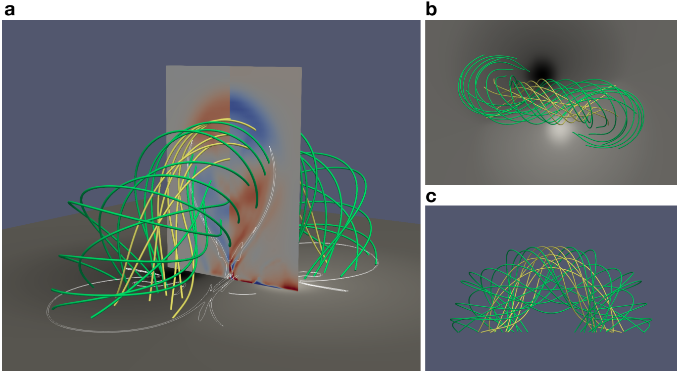
Figure S3. Magnetic field lines in the flux rope at t = 58 . (a) Forces on the plane y = 0 and field lines in the flux rope. The green (yellow) shows the highly (weakly) twisted field lines. In the plane y = 0 , the left half panel shows the z-component of the thermal pressure gradient force and the right half panel shows the z-component of the Lorentz force. The colors and the scales of the forces are the same as those in Fig. 6. The cell-center bottom surface shows the distribution of B_z . The white contours on the bottom surface and the vertical plane represent the contours of QSLs. (b) Top view of panel a. (c) Face-on view of panel a.
