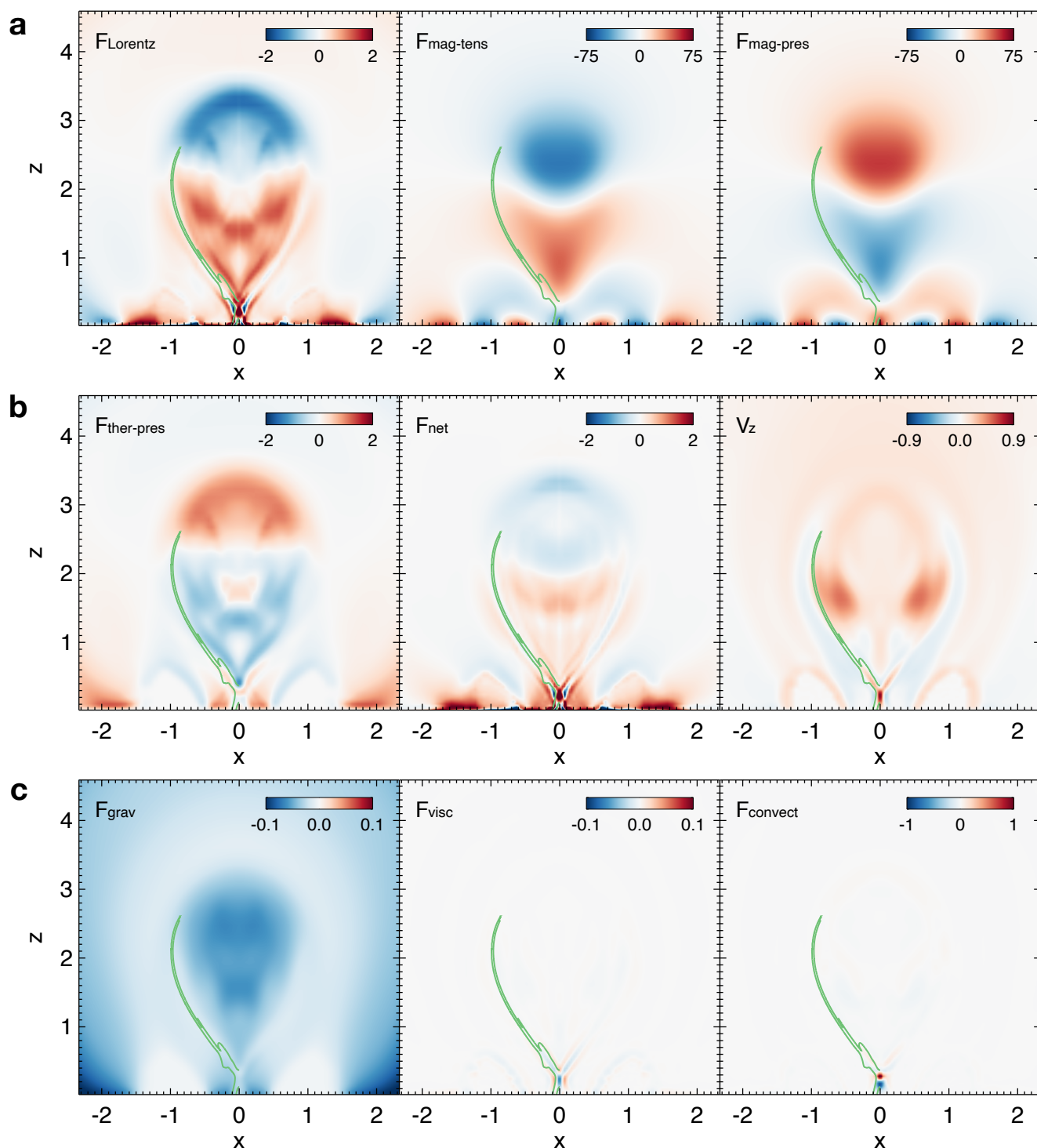
Figure 6. Component of forces and velocity in the z -direction in the plane y = 0 at t = 58 . They are in order as follows: Lorentz force ( F_{Lorentz} ), magnetic tension force ( F_{mag-tens} ), magnetic pressure gradient force ( F_{mag-pres} ), thermal pressure gradient force ( F_{ther-pres} ), net force ( F_{net} ), velocity ( v_z ), gravity ( F_{grav} ), viscous force ( F_{visc} ), and force related to the convection ( F_{convect} ). F_{net} is the sum of F_{Lorentz} , F_{ther-pres} , F_{grav} , and F_{visc} . Here the F_{mag-tens} ( F_{mag-pres} ) is derived by first decomposing \mathbf{B} \cdot \nabla \mathbf{B} ( -\nabla(B^2/2) ) to the normal direction of magnetic field and then further decomposing to the z -direction, given that the tangential component does not contribute to the acceleration. All of forces and velocity are in dimensionless units. The green contours represent the profiles of QSLs in the half panel of x \leq 0 . See Appendix B for more details for locating the flux rope boundary.
