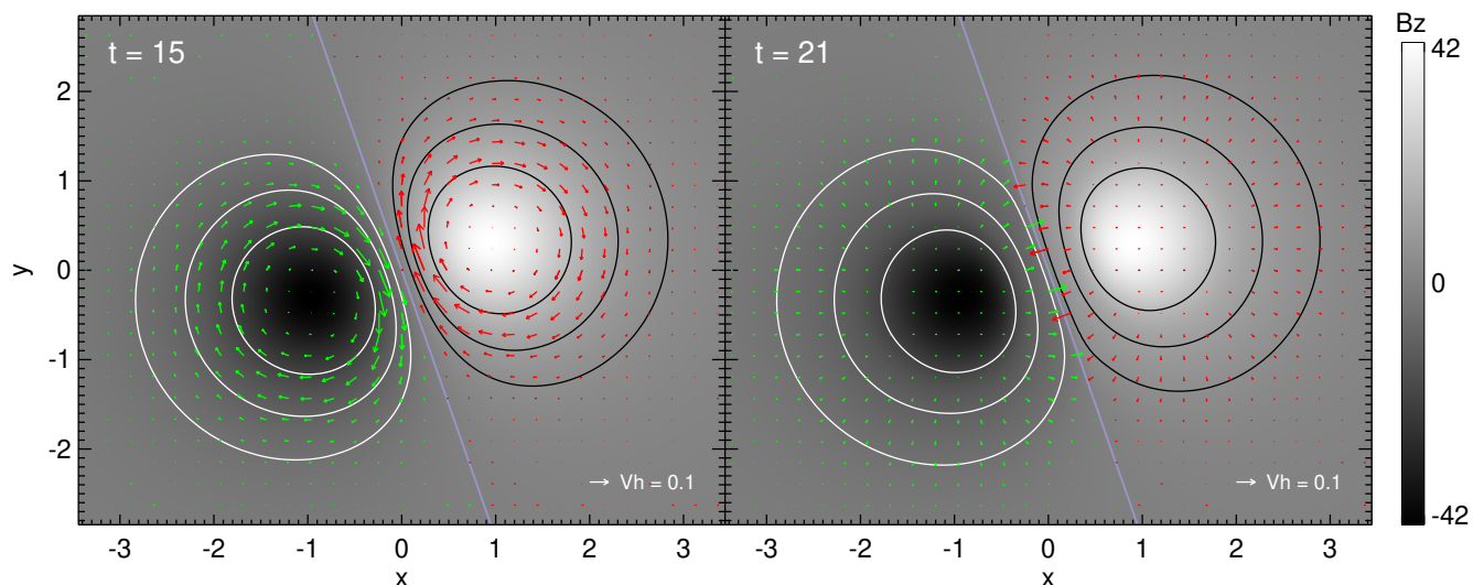
Figure 1. Distribution of B_z and imposed horizontal driving motions on the cell-center bottom surface. The black (white) contours in the positive (negative) polarity are the contours of B_z , and the purple ones show the PILs. The red (green) arrows in the positive (negative) polarity in the left panel show the shearing flow at t = 15 , and those in the right panel show the converging flow at t = 21 . The arrow orientation denotes the direction of the motion, and its length represents the magnitude of the speed ( v_h ). The scale of v_h is shown at the bottom right corner of each panel. All parameters are in dimensionless units.
