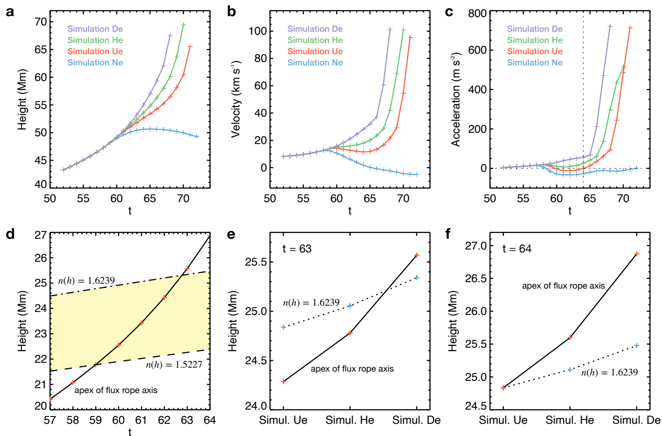
Figure S1. Kinematics of CME progenitors and CMEs in four simulations and estimation of the onset time of the torus instability in “Simulation De”. (a)-(c) Kinematics of CME progenitors and CMEs in “Simulation De” (purple curves), “Simulation He” (green curves), “Simulation Ue” (red curves), and “Simulation Ne” (blue curves). In panel c, the vertical and horizontal black dashed lines mark that the flux rope acceleration in “Simulation Ue” is close to zero at t = 64 . (d) The solid curve exhibits the height of the flux rope axis apex during 57 \leq t \leq 64 in “Simulation De”. The dotted-dashed curve (long-dashed curve) represents the evolution of the height ( h ) during 57 \leq t \leq 64 in “Simulation De”, the height which meets the condition that the decay index at (0, 0, h) equals 1.6239 (1.5227) at each moment. The yellow region marks the range for the critical height of the torus instability onset during 57 \leq t \leq 64 in “Simulation De”. (e) The solid curve shows the evolution of the height of the flux rope axis apex at t = 63 , from “Simulation (abbreviated as Simul.) Ue” to “Simulation He” to “Simulation De”. The dashed curve shows the evolution of the height ( h ), which meets the condition that the decay index at (0, 0, h) equals 1.6239 at t = 63 , from “Simulation Ue” to “Simulation He” to “Simulation De”. (f) Same as panel e but for those at t = 64 .
