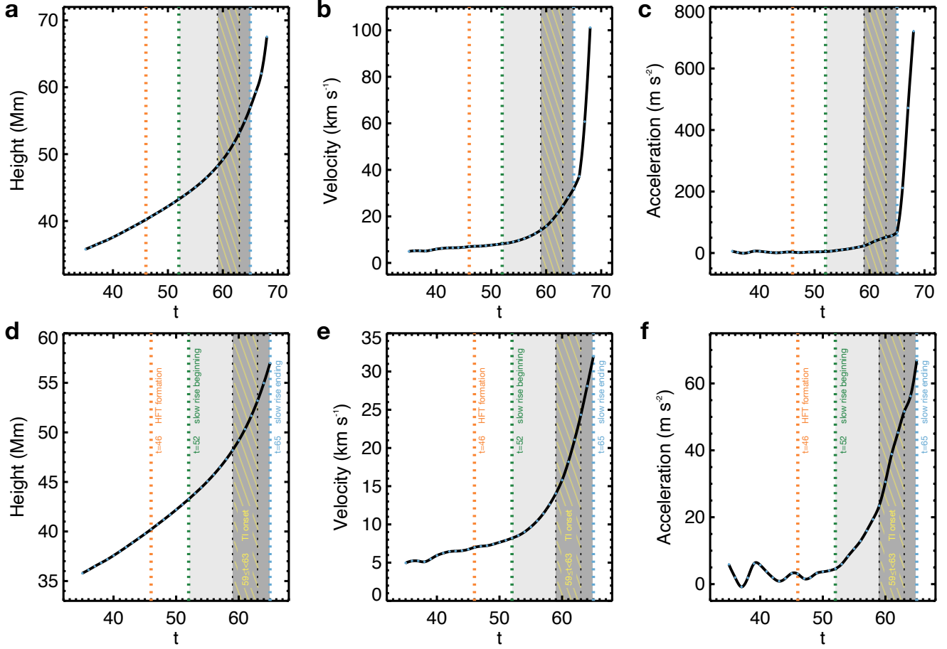
Figure 4. Kinematics of the CME progenitor and CME. (a)-(c) Kinematics of the CME progenitor and CME during 35 \leq t \leq 68 . In each sub-panel, the blue points show the measured or derived data and the black curve shows the fitting curve of data with the cubic spline interpolation method. The orange dashed line represents the time when the HFT first appears. The green and blue dashed lines mark the beginning and the end of the slow rise phase, respectively. The light grey and dark grey regions show the earlier stage and the later stage of the slow rise phase, respectively. The two black dashed lines and the yellow oblique-line-region between them mark the time range of the torus instability onset. (d)-(f) Same as panels a-c but for the kinematics during 35 \leq t \leq 65 .
