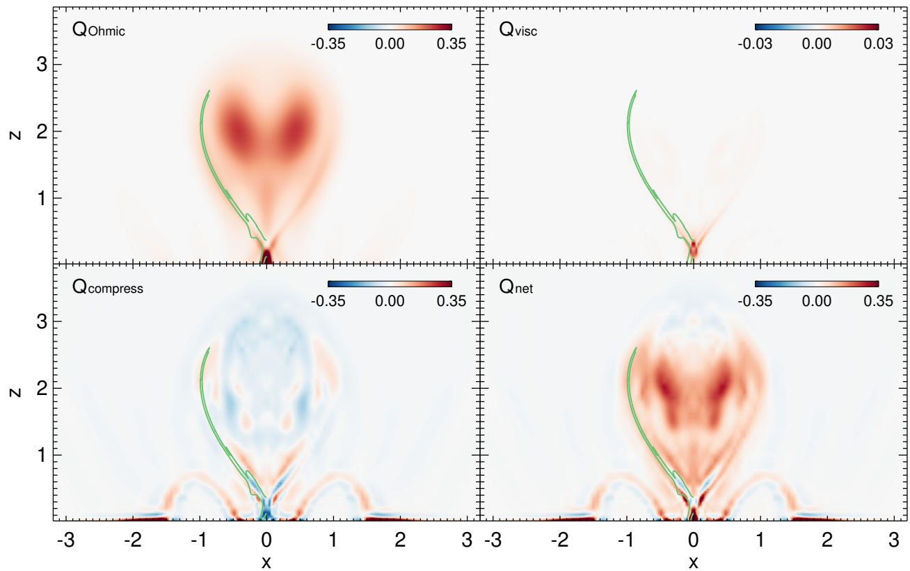
Figure 11. Heating rates on the plane y = 0 at t = 58 . They are in order as follows: rates of Ohmic heating ( Q_{Ohmic} ), viscous heating ( Q_{visc} ), compression heating ( Q_{compress} ), and net heating ( Q_{net} ) which is the sum of the first three. All heating rates are in dimensionless unit. The field of view is the same as that of the synthetic image along the y -direction in Fig. 2a. The green contours represent those of QSLs at the half panel of x \leq 0 .
